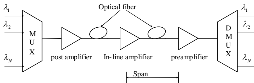
Fig.1 Implementation of a typical WDM network containing various types of optical amplifiers.
